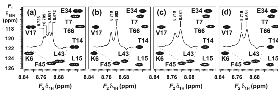
Fig. 4 Partial ^1\text{H} - ^{15}\text{N} -HSQC spectra of ^{15}\text{N} -ubiquitin in 90 % \text{H}_2\text{O}/10 % \text{D}_2\text{O} ( 2 ) acquired by using a HSQC, b HSQC with CAWURST homonuclear decoupling during acquisition, c pure shift gBIRD-HSQC and d pure shift gBASHD-HSQC
